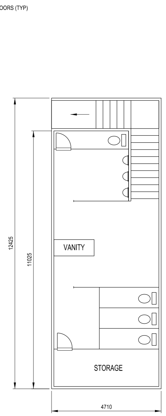
DETAIL 1 1:100
